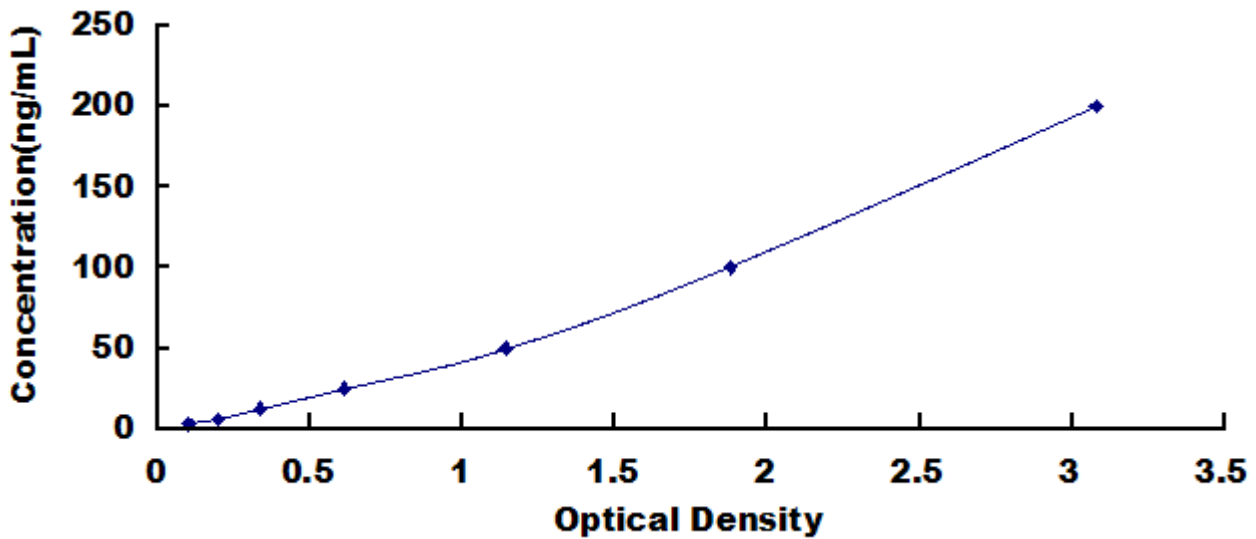
Typical Standard Curve for Lysozyme, Human ELISA.
