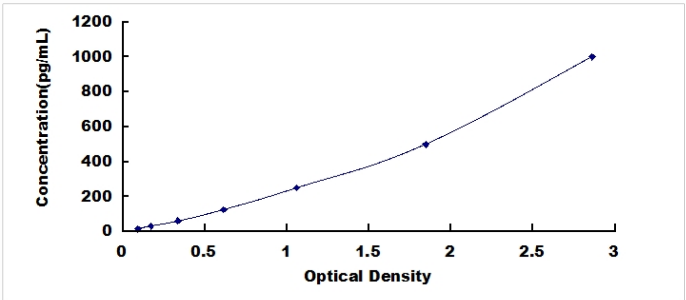
Typical Standard Curve for MIP1a, Human ELISA.
