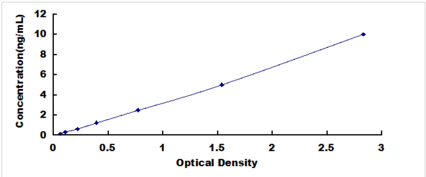
Typical Standard Curve for Meteorin, Mouse ELISA.
