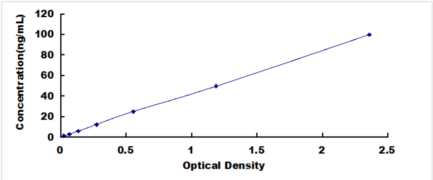
Typical Standard Curve for METRNL, Human ELISA.
