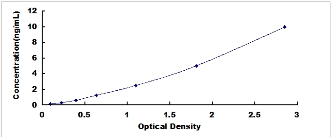
Typical Standard Curve for MECR, Human ELISA.
