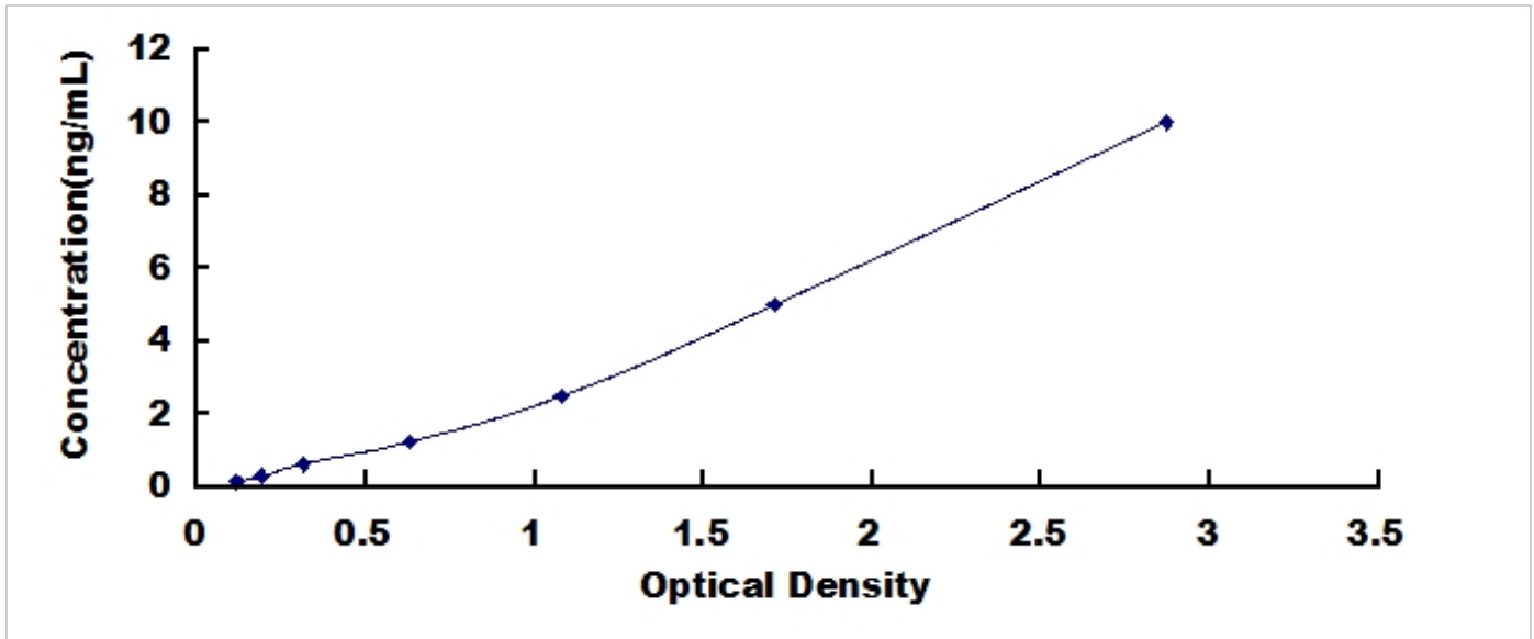
Typical Standard Curve for MAP2K1, Human ELISA.
