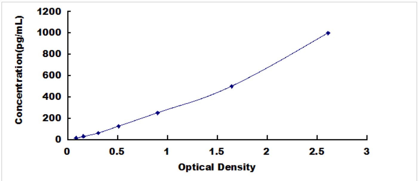
Typical Standard Curve for MCP2, Bovine ELISA.
