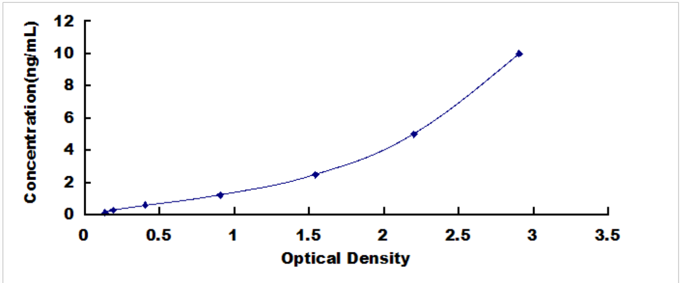
Typical Standard Curve for MBP, Rat ELISA.
