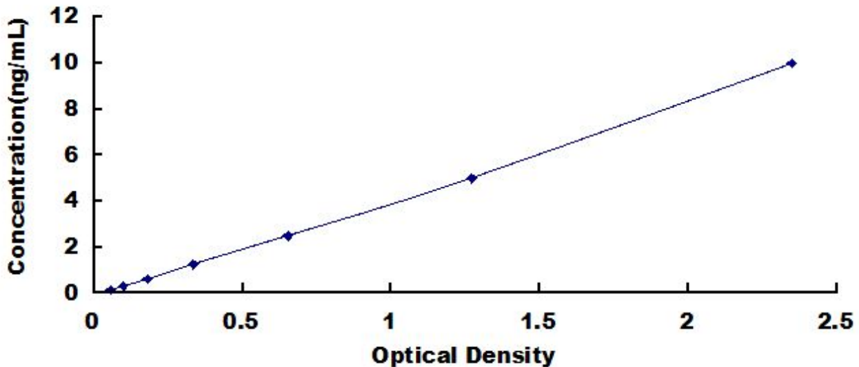
Typical Standard Curve for MyoD, Human ELISA.
