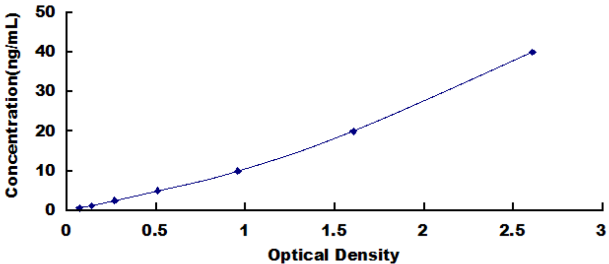
Typical Standard Curve for Myoglobin, Rat ELISA.
