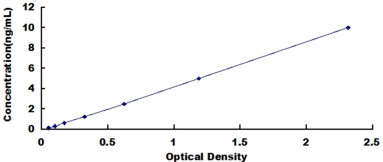
Typical Standard Curve for MARCKS, Human ELISA.
