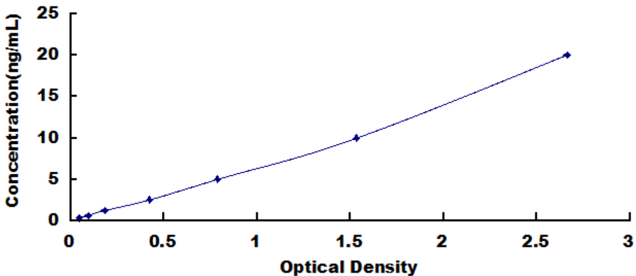
Typical Standard Curve for N4BP2, Human ELISA.
