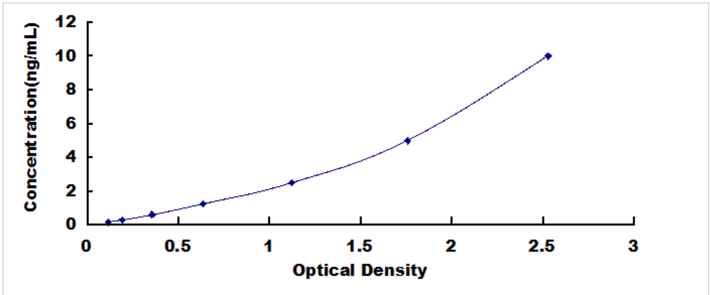
Typical Standard Curve for NRN1, Mouse ELISA.
