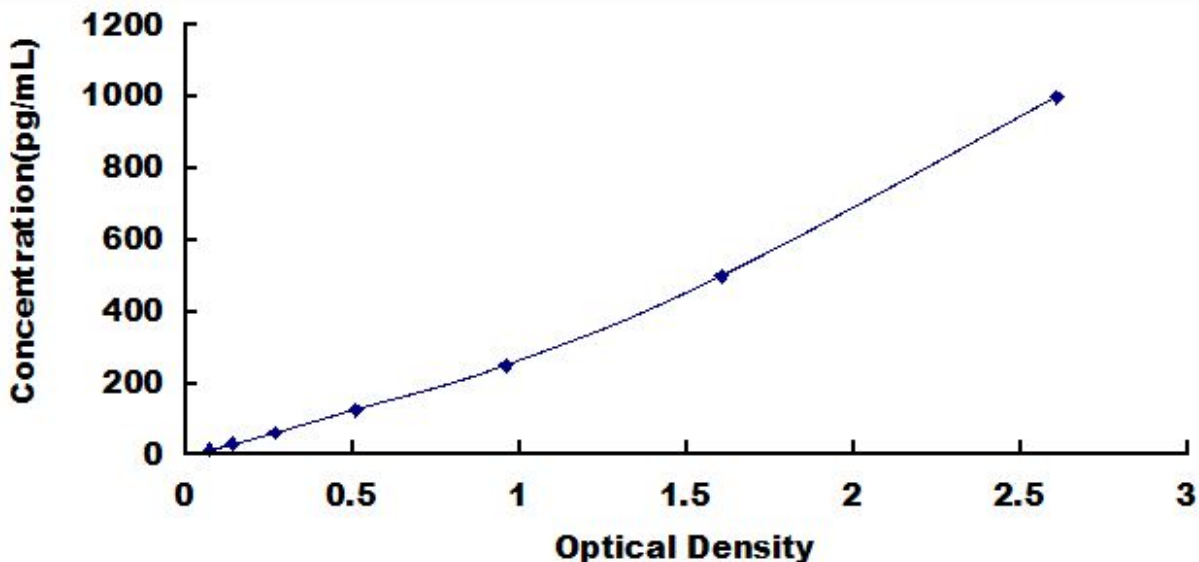
Typical Standard Curve for NEFH, Human ELISA.
