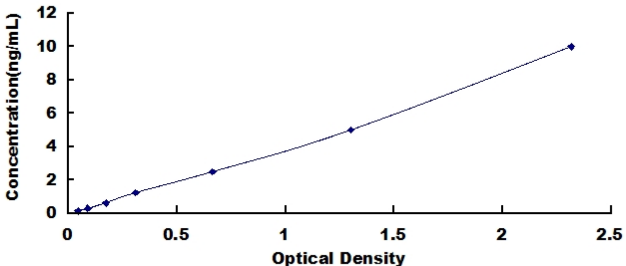
Typical Standard Curve for NPTX1, Mouse ELISA.
