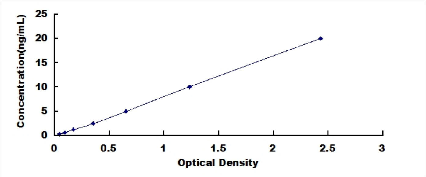
Typical Standard Curve for NPC1, Human ELISA.
