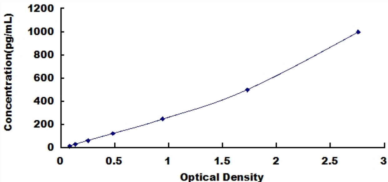
Typical Standard Curve for OSM, Human ELISA.
