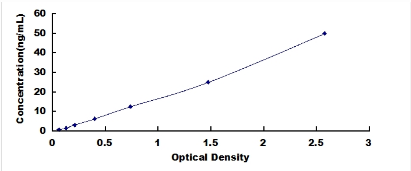
Typical Standard Curve for Ovalbumin ELISA.
