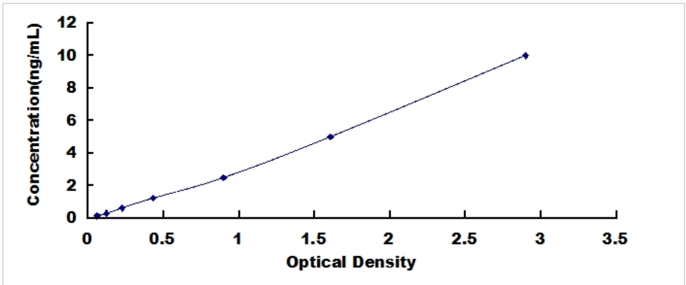
Typical Standard Curve for OXSR1, Human ELISA.
