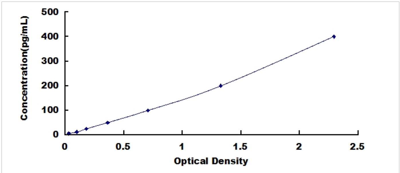
Typical Standard Curve for PF4, Bovine ELISA.
