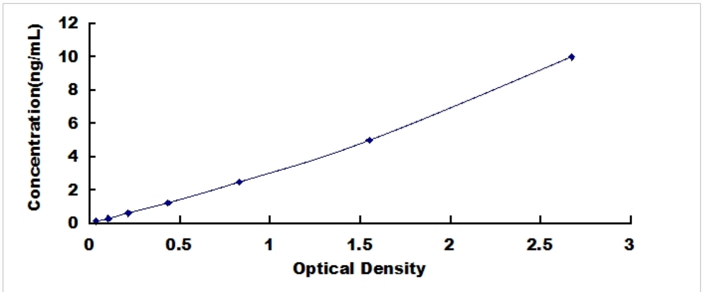
Typical Standard Curve for Pleckstrin, Human ELISA.
