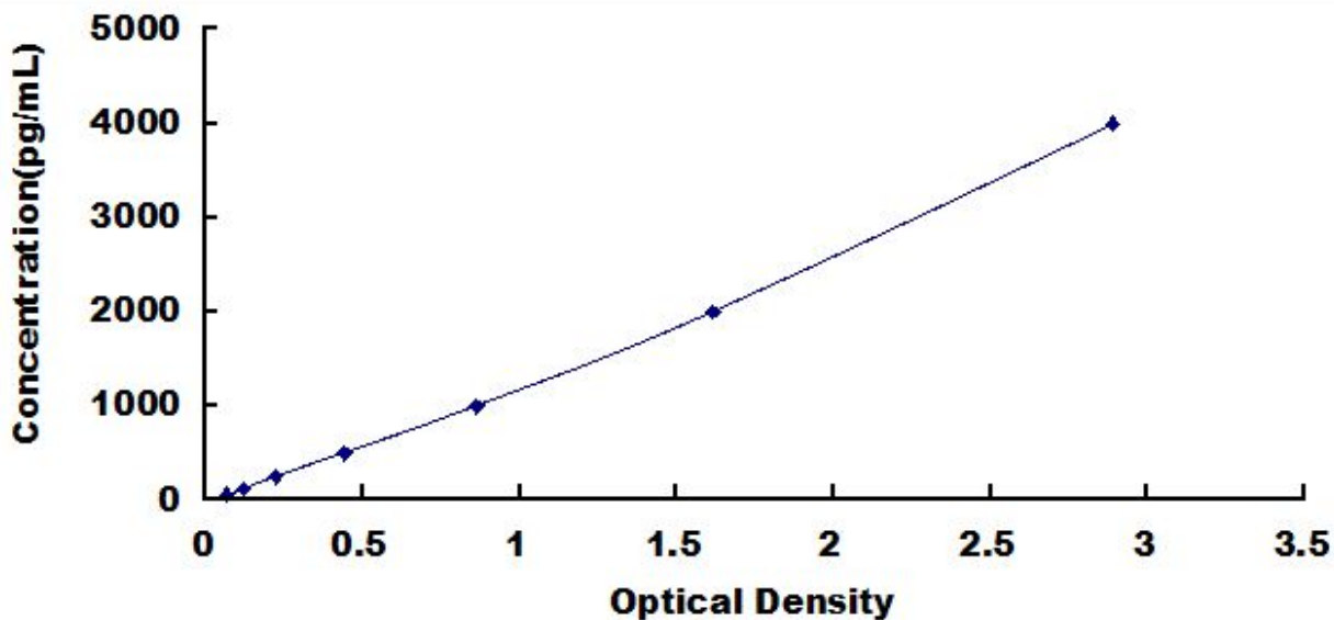
Typical Standard Curve for PIGR, Human ELISA.
