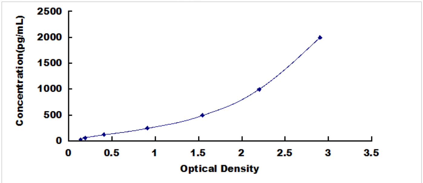
Typical Standard Curve for PIICP, Human ELISA.
