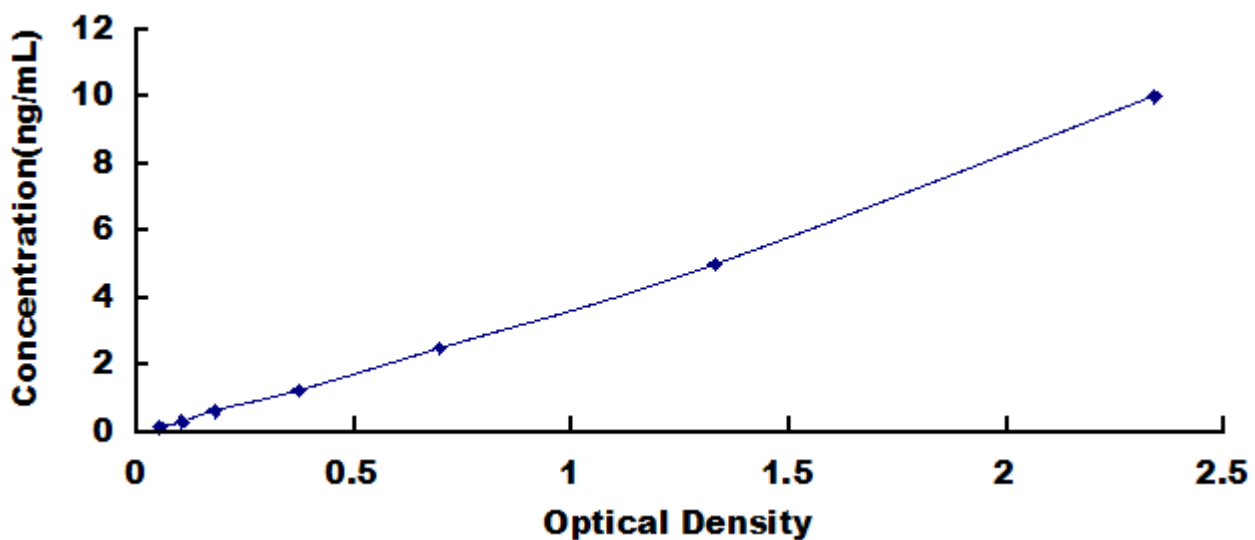
Typical Standard Curve for KLK3, Rat ELISA.
