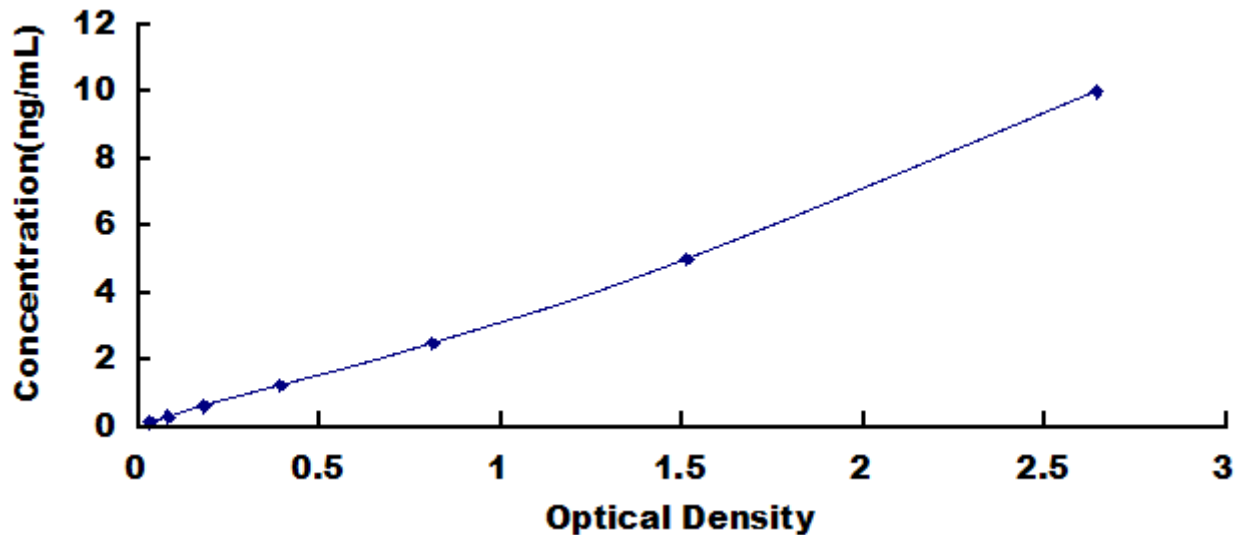
Typical Standard Curve for PSMA1, Human ELISA.
