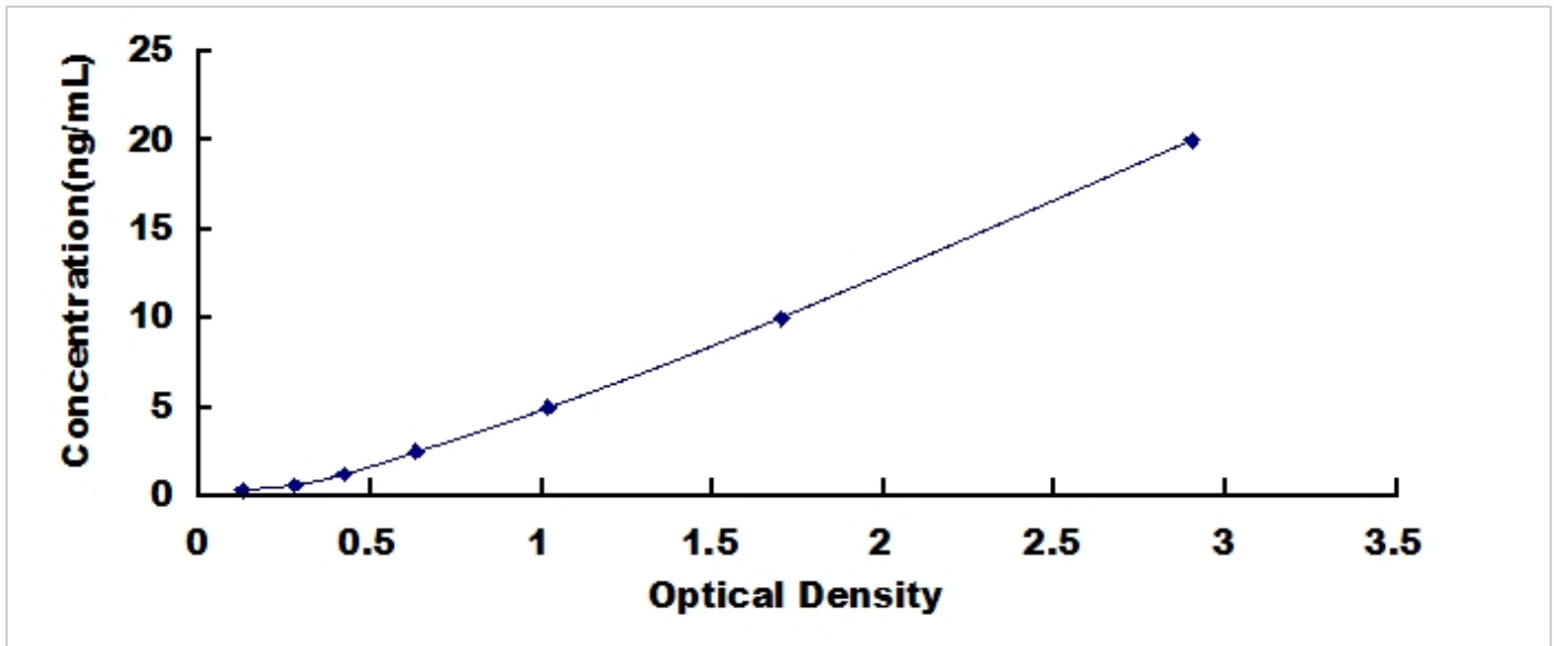
Typical Standard Curve for PRKDC, Mouse ELISA.
