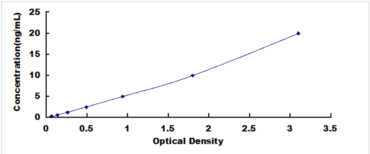
Typical Standard Curve for P2RX4, Human ELISA.
