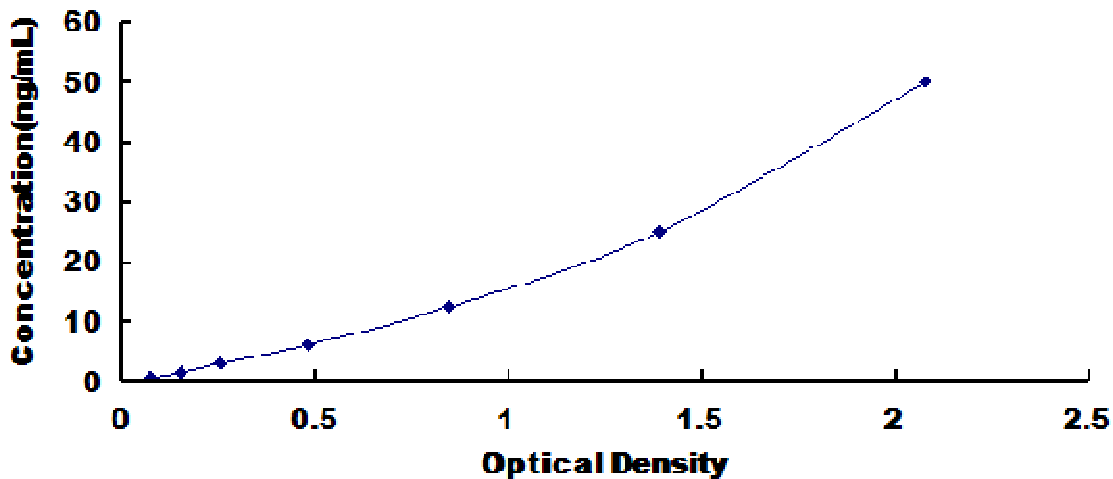
Typical Standard Curve for PK, Rat ELISA.
