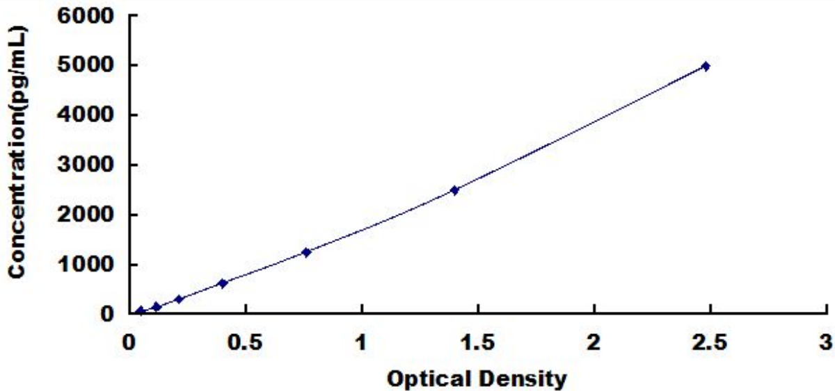
Typical Standard Curve for PKM2, Human ELISA.
