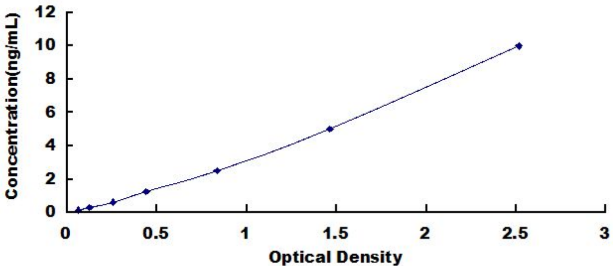
Typical Standard Curve for RASA1, Human ELISA.
