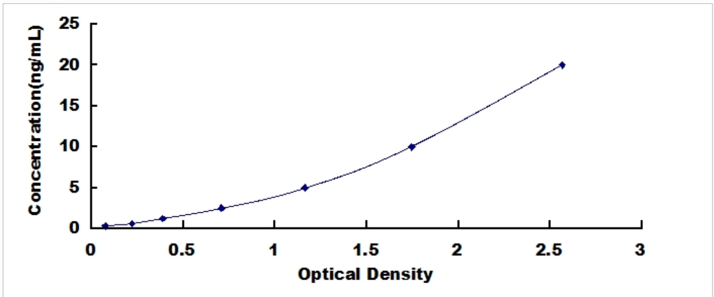
Typical Standard Curve for ROMO1, Bovine ELISA.
