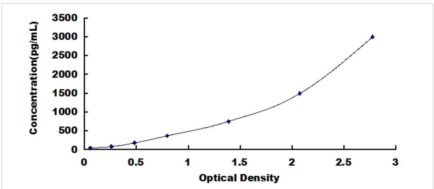
Typical Standard Curve for FcgRII, Human ELISA.
