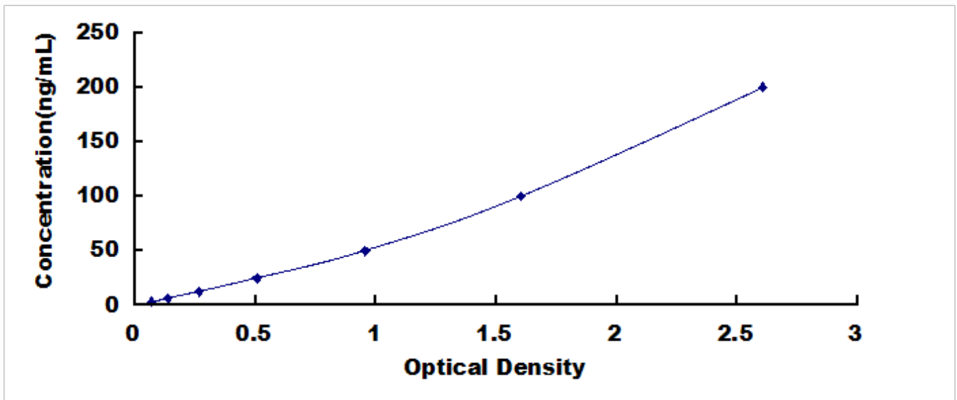
Typical Standard Curve for RANTES, Porcine ELISA.
