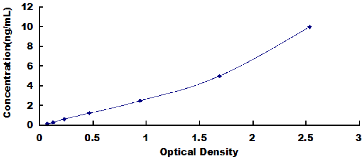
Typical Standard Curve for RPLP2, Human ELISA.
