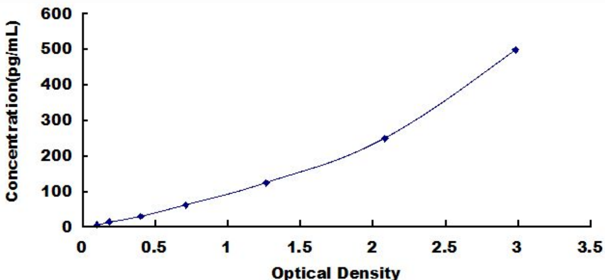
Typical Standard Curve for S100A8, Mouse ELISA.
