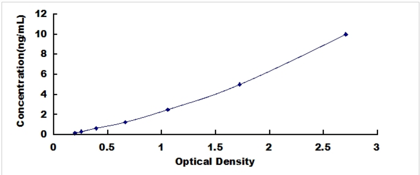
Typical Standard Curve for SEC24C, Human ELISA.
