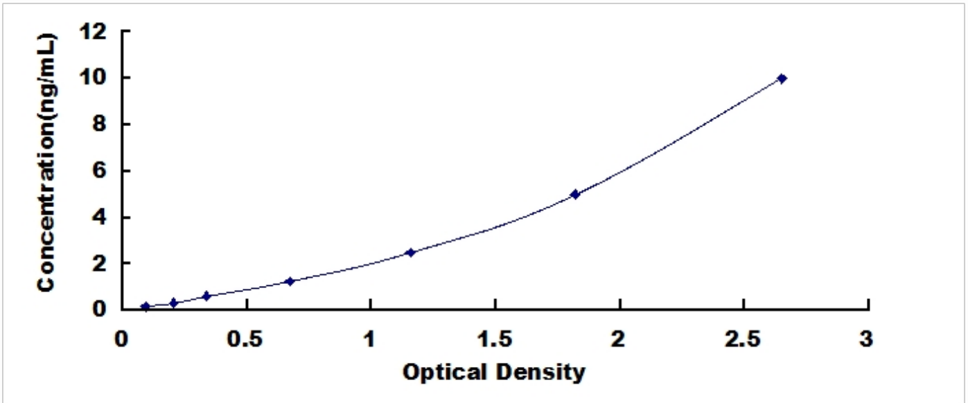
Typical Standard Curve for SMOC1, Human ELISA.
