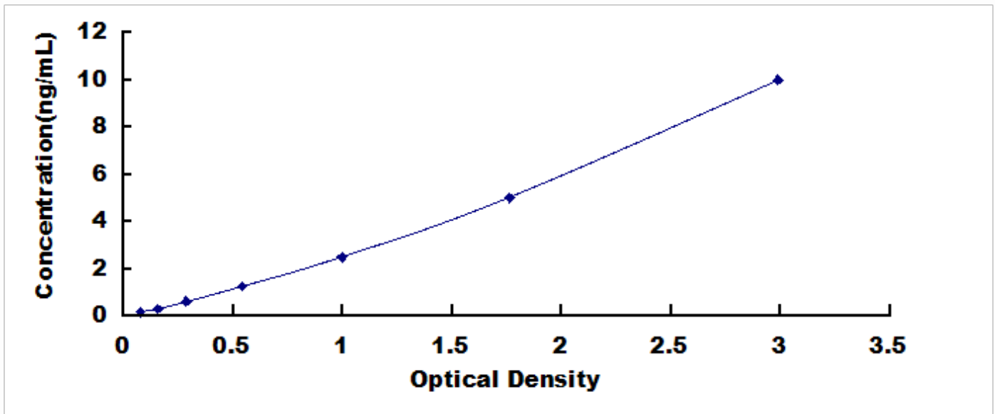
Typical Standard Curve for SCXB, Human ELISA.
