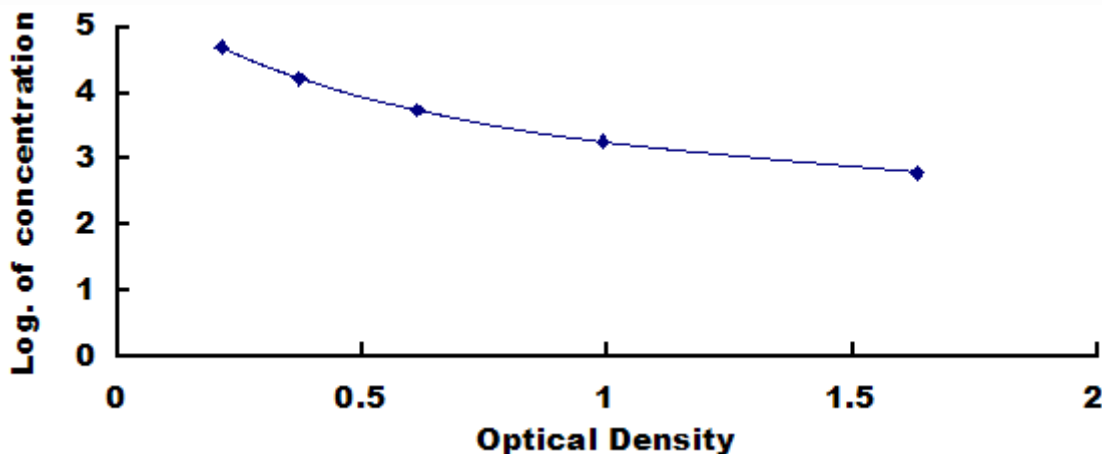
Typical Standard Curve for sIgA, Gallus ELISA.
