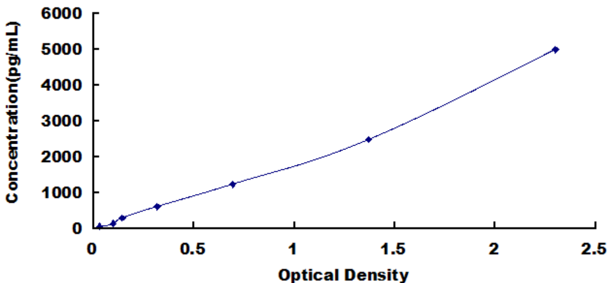
Typical Standard Curve for SEMA4B, Mouse ELISA.
