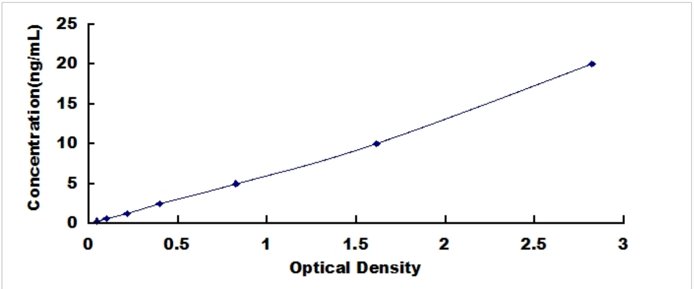
Typical Standard Curve for SPINT2, Human ELISA.
