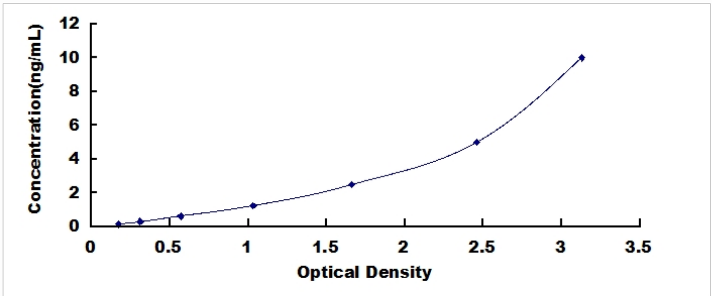
Typical Standard Curve for SIAT1, Human ELISA.
