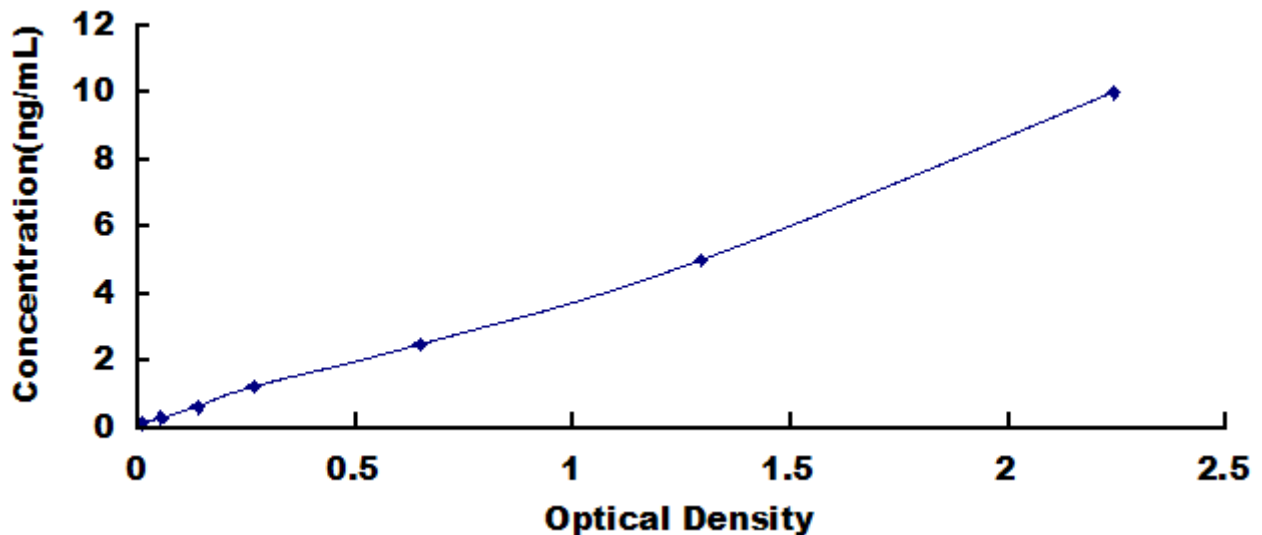
Typical Standard Curve for SPRR1A, Human ELISA.
