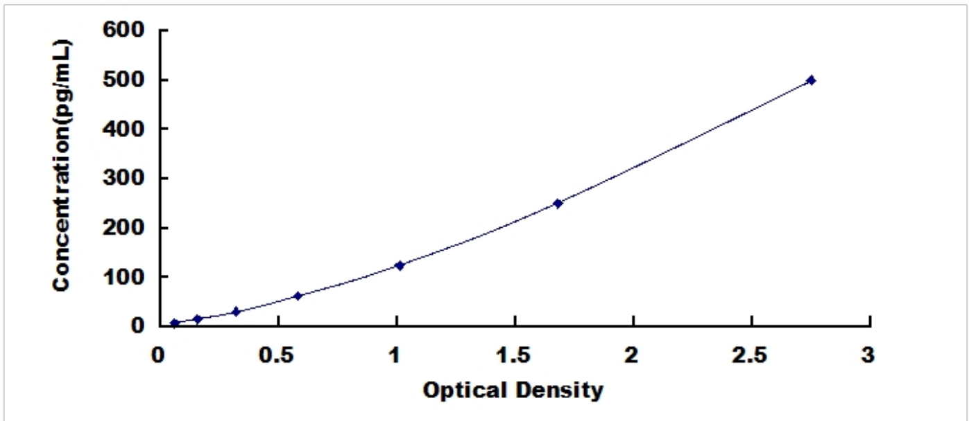
Typical Standard Curve for SST, Mouse ELISA.
