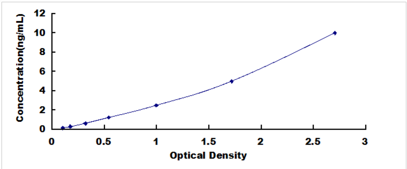
Typical Standard Curve for SPAM1, Mouse ELISA.
