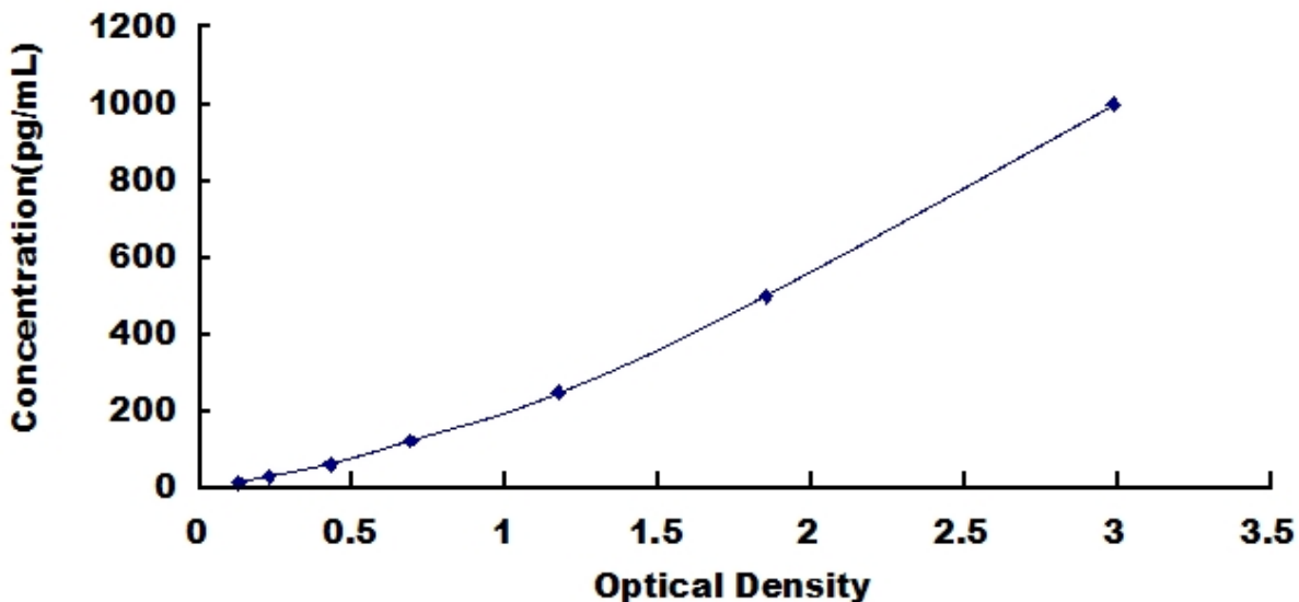
Typical Standard Curve for SCF, Human ELISA.
