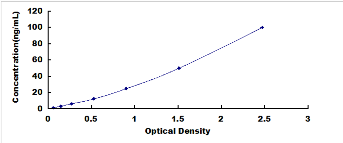
Typical Standard Curve for SPB, Human ELISA.
