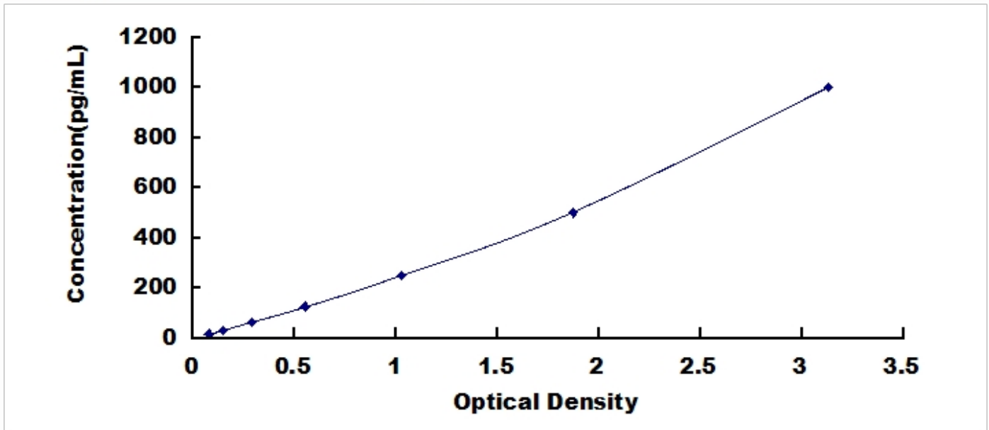
Typical Standard Curve for Survivin, Mouse ELISA.
