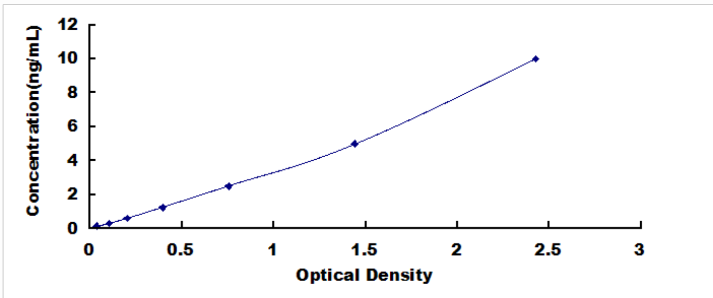
Typical Standard Curve for Tafazzin, Human ELISA.
