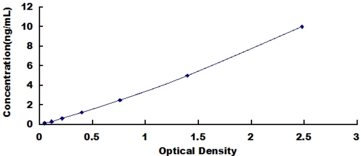
Typical Standard Curve for THSD7A, Human ELISA.
